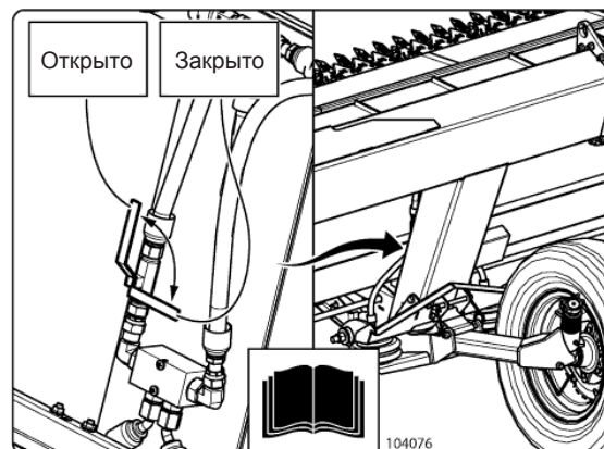
Рис. 130 - Gauge wheel isolation valve
